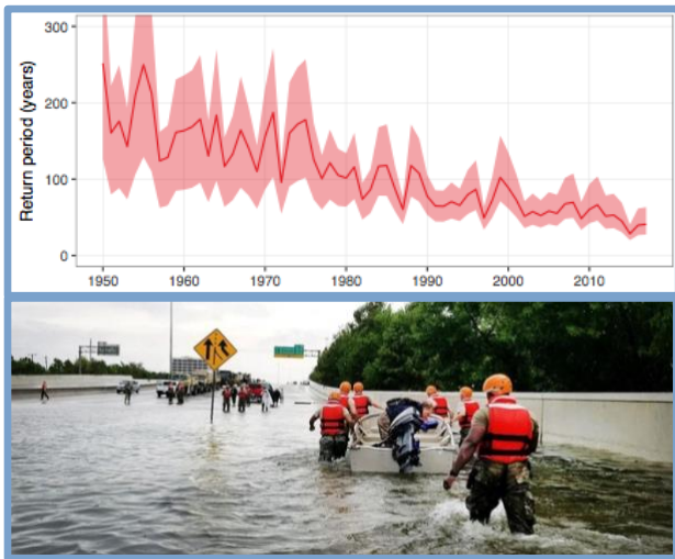
Extreme weather events, such as flooding caused by Hurricane Harvey in 2017 (bottom), are used as case-studies for understanding how impactful hurricanes are changing. Analysis of observations (red line), and consideration of uncertainty (red shading) indicate that storms like Hurricane Harvey are becoming much more common.
